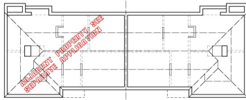
ROOF SPACE PLAN THE BUNGLOW BRIERFIELD
